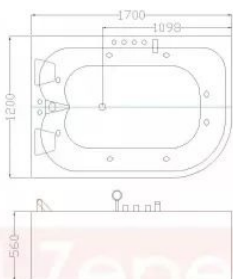
Wanna model LS-7001
